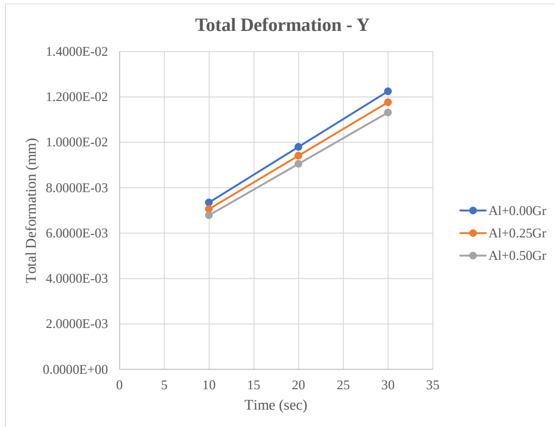
Figure: 9 total Deformation in Y Direction.
