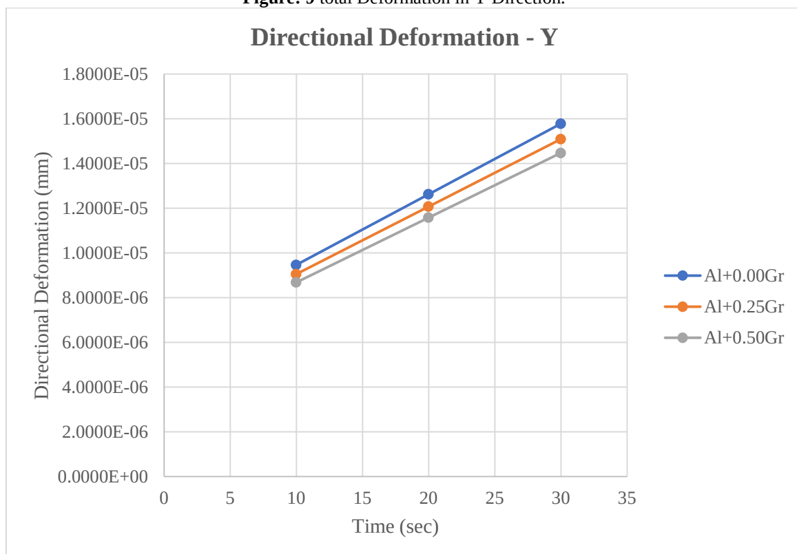
Figure 10: Directional deformation in Y Directional
