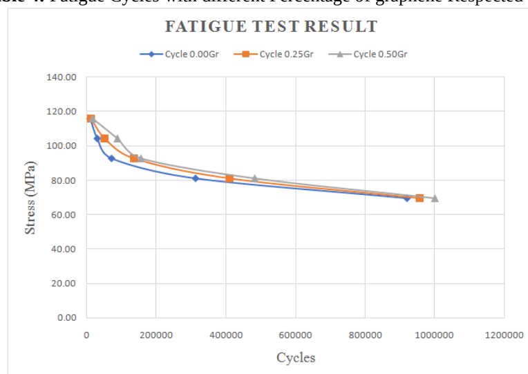
Figure 7: Fatigue Test Result Graph- Stress Vs cycles.
