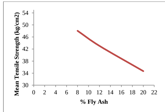
Figure 5: Representation of Tensile Strength w.r.t. % Fly Ash Content
