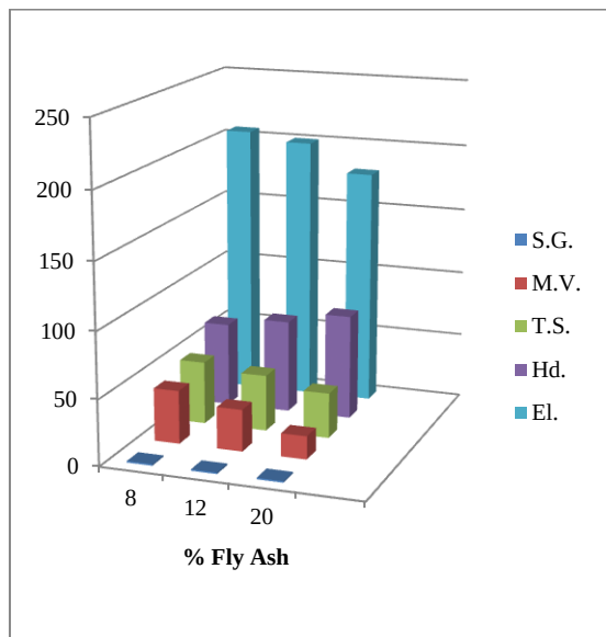
Figure 4: Representation of mechanical properties w.r.t. % Fly Ash Content
