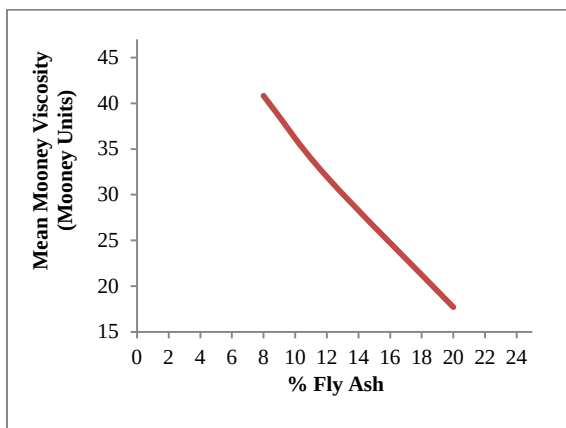
Figure 7: Representation of Mooney Viscosity w.r.t. % Fly Ash Content
