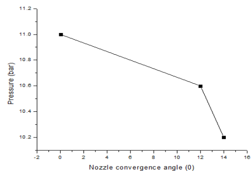
Pressure vs Nozzle converging angles
