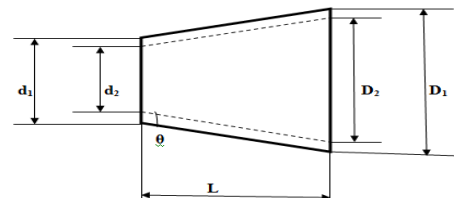
1. Line diagram of diffuser 1. Diffusers
